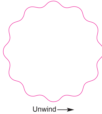
Die #792 1 3/4" DIA.
